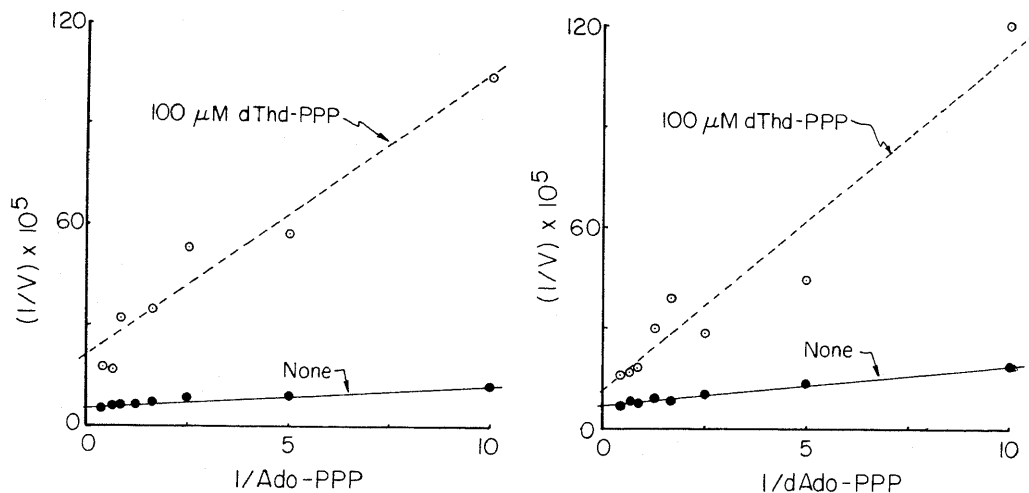
FIGURE 3. Double reciprocal plots of reaction velocity V versus phosphate donor concentrations for Step 8 enzyme with and without dThd-PPP. Concentrations of dThd and dThd-PPP were 400 and 100 \mu M, respectively; other conditions were as described in Methods. Correlation coefficients for Ado-PPP and dAdo-PPP alone were 0.98 and 0.99, respectively, and for these nucleoside triphosphates in the presence of dThd-PPP were 0.97 and 0.97, respectively.
